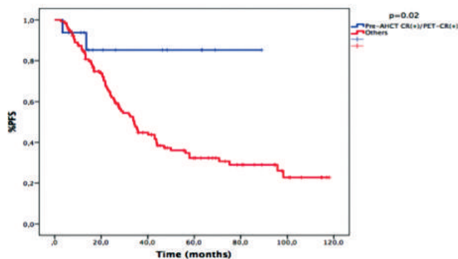
Figure 1: Impact of Pre-AHCT and Post-AHCT CR and PET-CR on PFS curves
