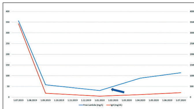
Figure 2. Case B IgA and free Lambda Levels
