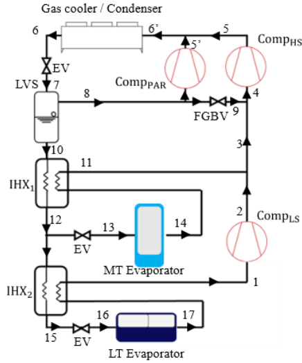
Figure 1. The schematic of the system.
