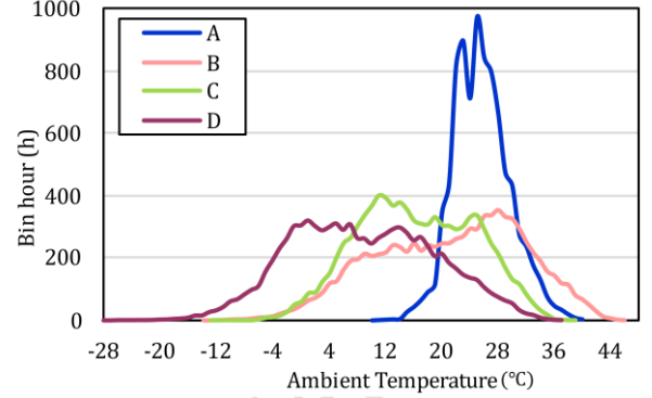
Figure 3. Bin-hour modeling for different climates
