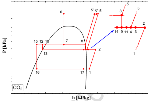
Figure 2. P-h diagram of the system.
