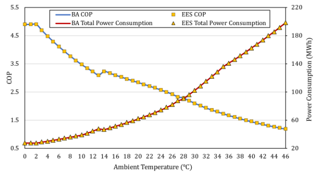
Figure 9. Optimized power consumption and COP values for each ambient temperature.
