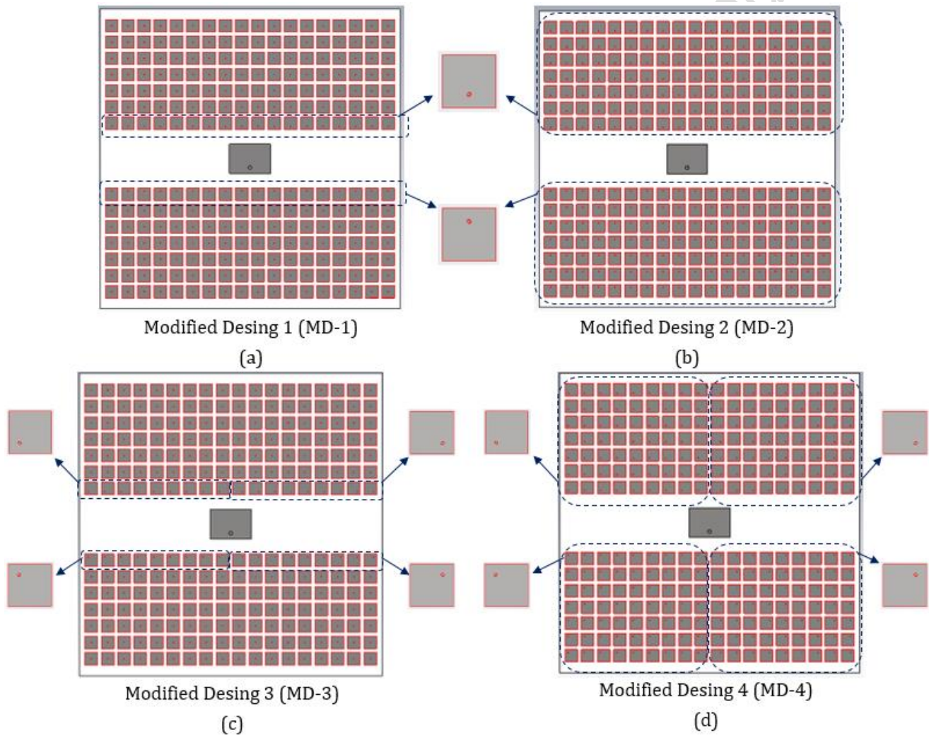
Fig. 4. The illustrations of the Modified Designs.
