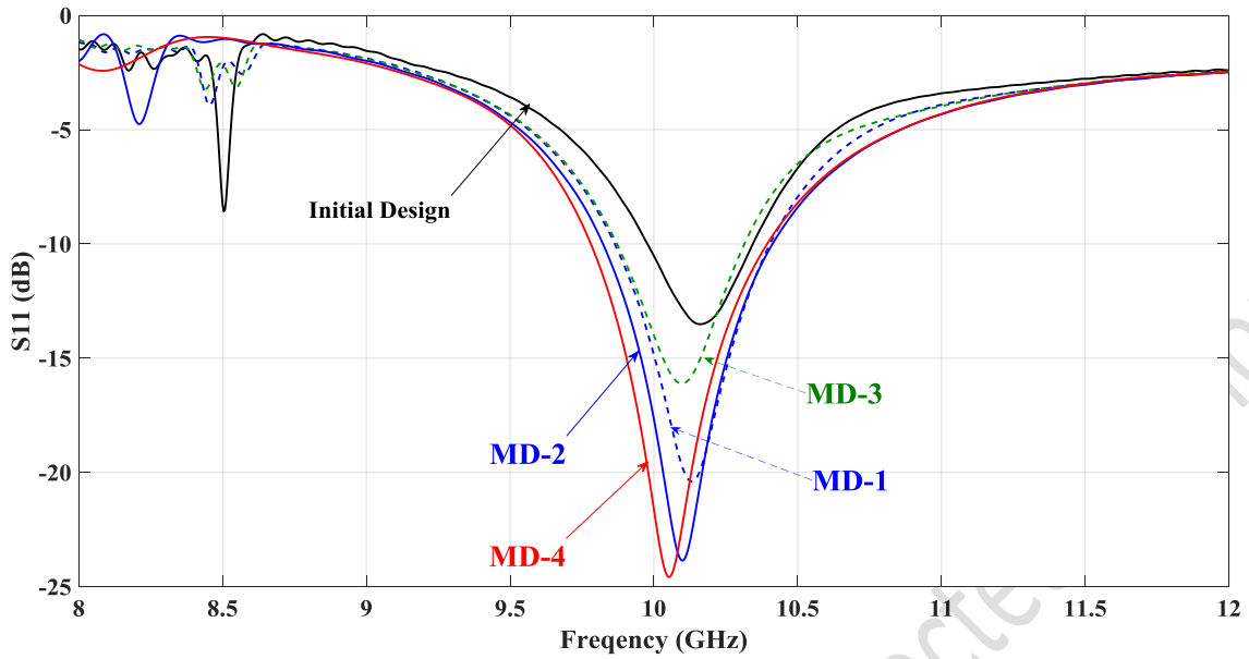
Fig. 5. The simulated S11 (reflection coefficient) results for different designs with offset vias.
