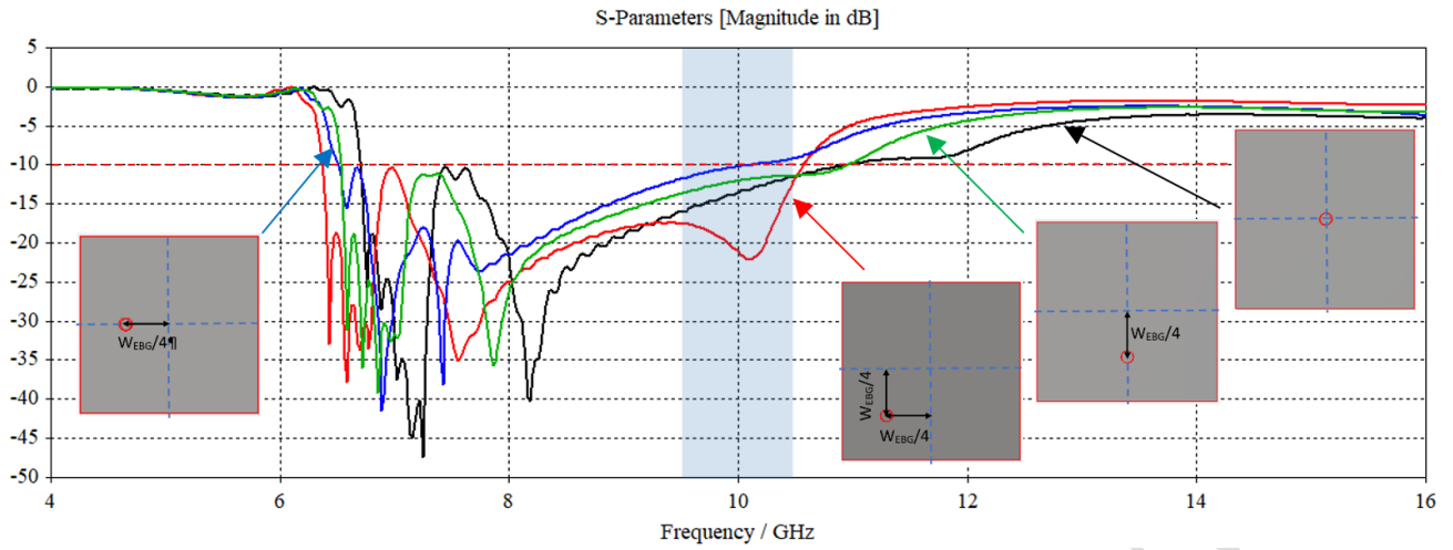
Fig. 3. The simulated S21 (transmission coefficient) results for offset vias in only x, only y and both x and y directions for 4x4 arrays.
