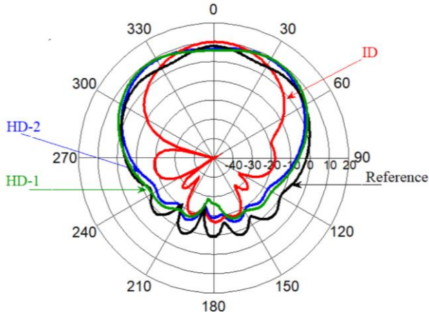
Figure 9. Gain patterns of the HD-1 and HD-2 in comparison with the reference antenna and ID.
