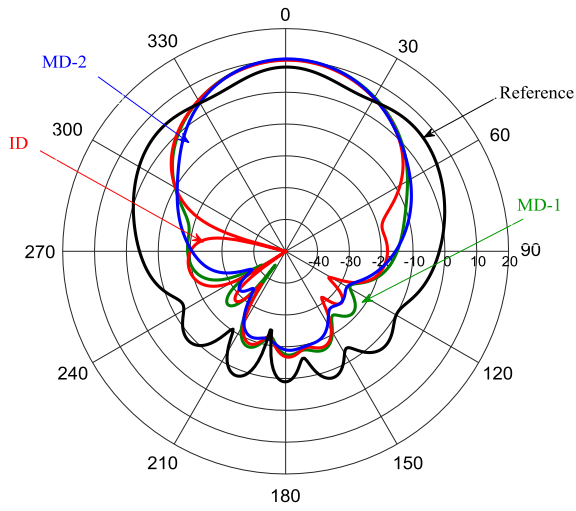
(a) MD-1, MD-2
