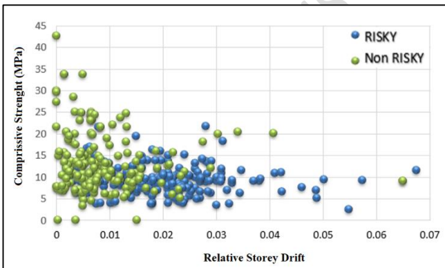
Figure 5. Concrete compressive strength-Storey drift relationship.
