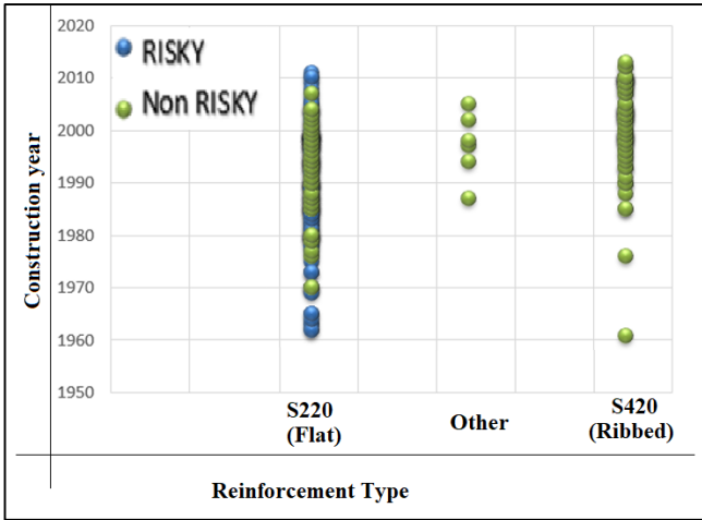
Figure 4. Construction year vs. reinforcement type graph.
