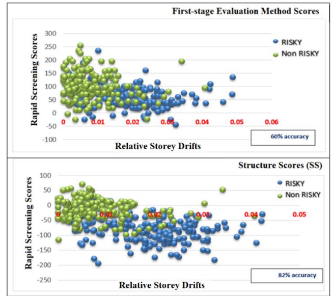
Figure 3. Comparison of the Structure Score method and the First-stage Valuation Method.
