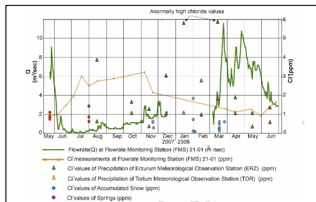
Figure 4. The change of chloride content in the samples through sampling period.
