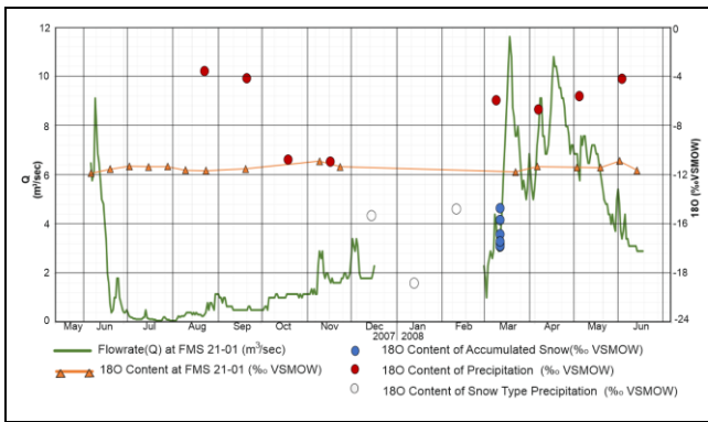
Figure 5. The change of \delta^{18}\text{O} content in samples through the sampling period.
