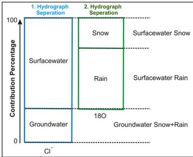
Figure 3. Two-stage hydrograph separation model.
