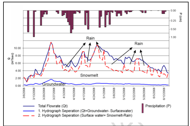
Figure 6. Hydrograph separations.
