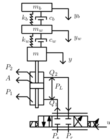
Figure 1. Schematic representation of the hydraulic road test system.
