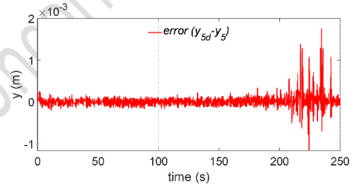
Figure 12. Error between piston displacement and RRI 3.
