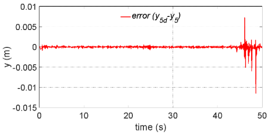
Figure 9. Error between piston displacement and RRI 2.
