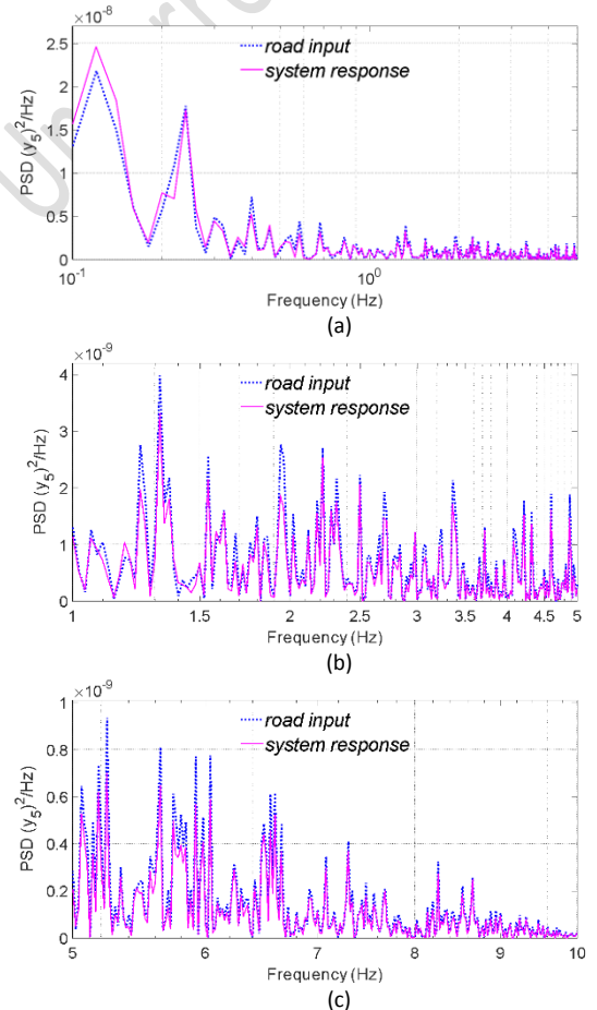
Figure 7. Piston displacement and RRI 1 (frequency domain) (a) 0.1-10 Hz interval (b) 1-5 Hz interval (c) 5- 10 Hz interval.
