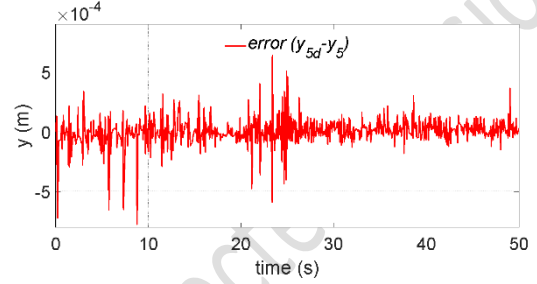
Figure 6. Error between piston displacement and RRI 1.
