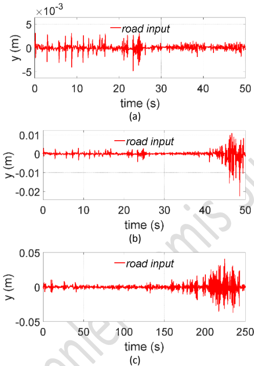
Figure 4. Road references (a) RRI 1 (b) RRI 2 (c) RRI 3.
