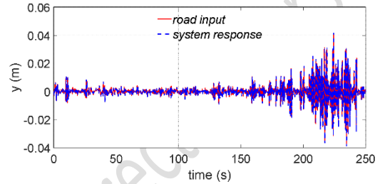
Figure 11. Piston displacement and RRI 3.
