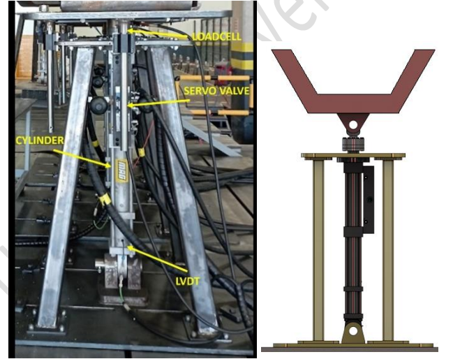
Figure 2. Experimental apparatus.
