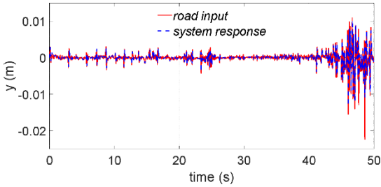
Figure 8. Piston displacement and RRI 2.
