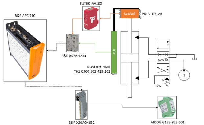
Figure 3. Structure of the test rig.
