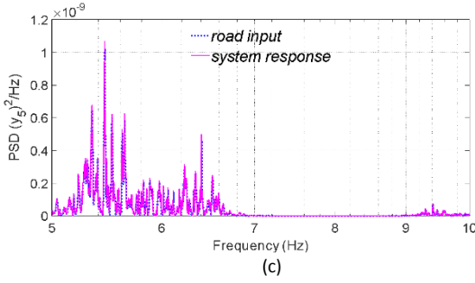
Figure 13. Piston displacement and RRI 3(frequency domain) (a) 0.1-10 Hz interval (b) 1-5 Hz interval (c) 5- 10 Hz interval.
