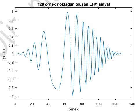
Şekil 4. 128 örnek noktadan oluşan LFM sinyali Figure 4. LFM Signal consisting of 128 sample points.
