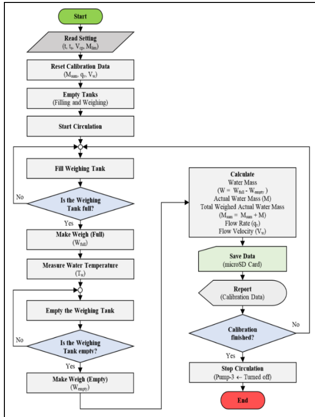
Figure 4. Flowchart for the microcontroller software algorithm.
