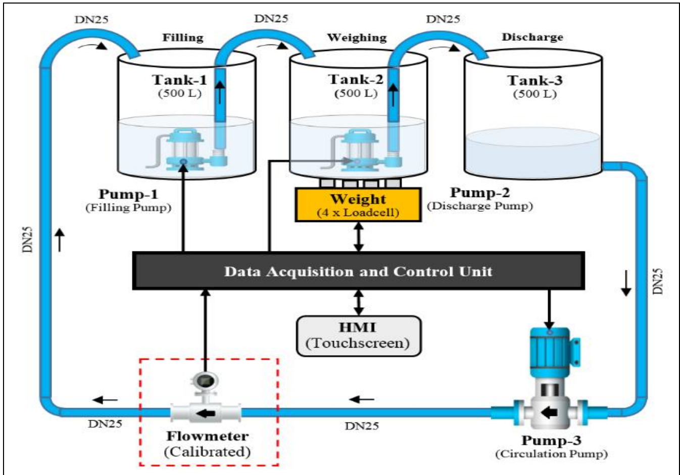
Figure 1. Infinite cycle calibration system basic principle.
