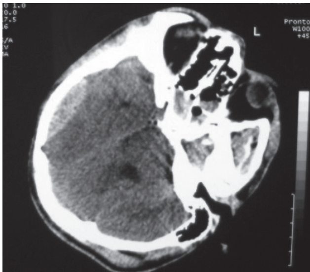
Fig. 1. Axial CT scan without contrast obtained on admission shows convex hematoma in the right epidural space.
