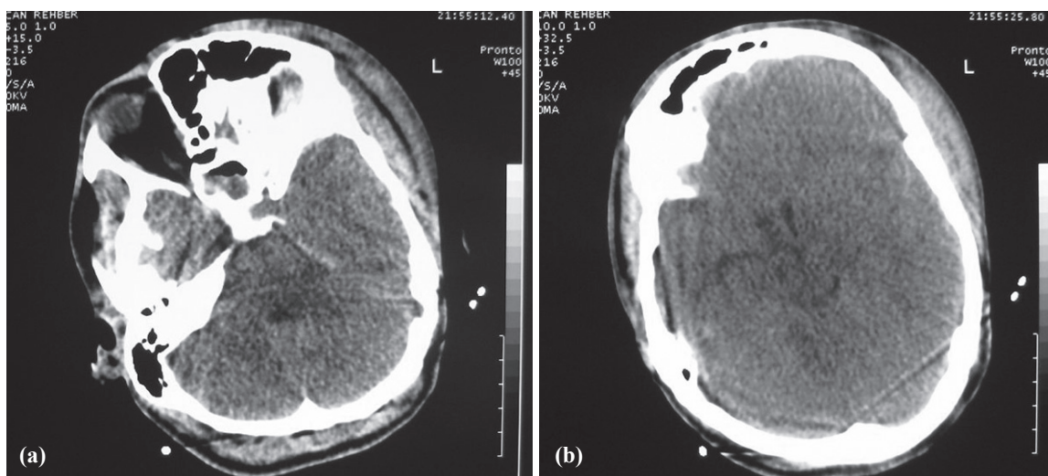
Fig. 2. (a) Same level axial CT scan as seen in Fig. 1 does not demonstrate epidural hematoma localization because the patient's head was not in the same position as in the first CT scan. The head was turned to nearly the opposite side, and the slice shows right mastoid cells and right orbita clearly. (b) Axial CT scan without contrast obtained 3 hours after injury shows almost total disappearance of the hematoma. This cross-section is not at the same level as seen in Fig. 1 because the patient's head position was altered on each CT slice. In fact, this slice shows the true epidural hematoma area, which had resolved almost totally in 3 hours.
