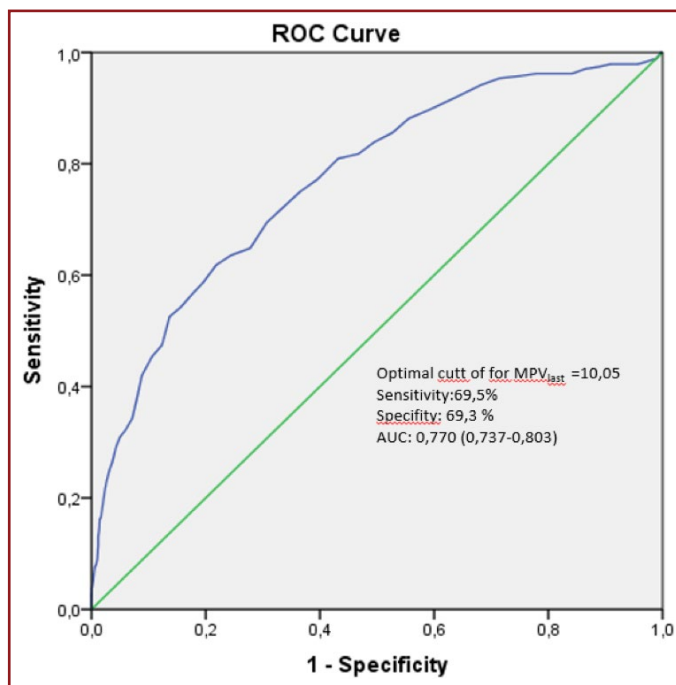
Figure 1. Receiver-operating characteristic curve of MPVlast predicting mortality.
